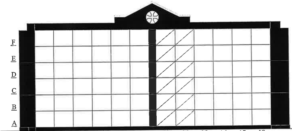
7 8 9 10 11 12 13 14 15 16 17 18 36 SINGLE CRYPTS 12 DOUBLE DEPTH CRYPTS 24 SINGLE CRYPTS ELEVATION 131
